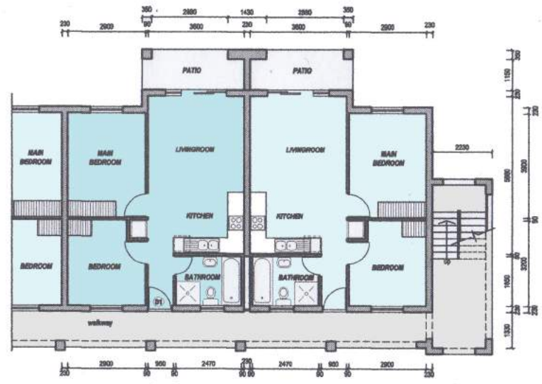
UNIT D FLOOR PLAN
